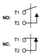
Auxiliary contacts (optional)
